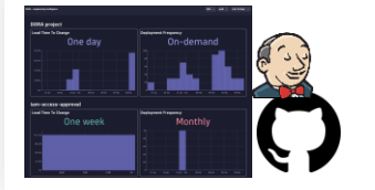
Out-of-the-box dashboards for engineering KPIs (DORA) with events from GitHub, ArgoCD, Jenkins
